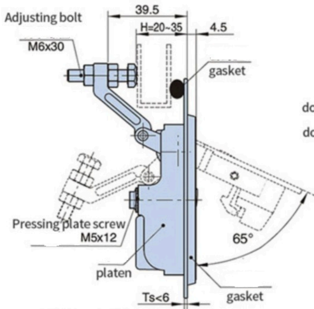
The pressing plate screws adapt to the thickness of the door panel
